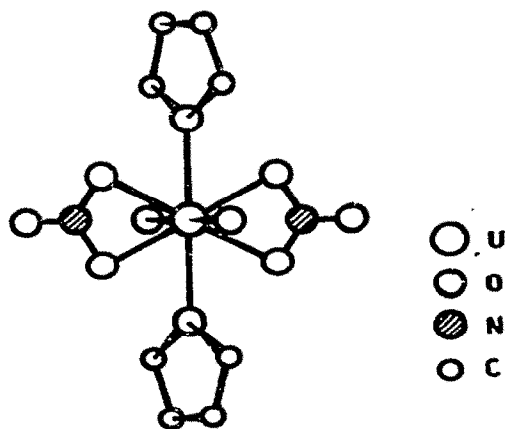
Fig. 20. The molecular structure of \text{UO}_2(\text{NO}_3)_2(\text{THF})_2 .
