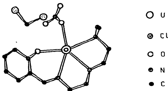
Fig. 34. Projection of the complex [\text{UO}_2(\text{o-O-C}_6\text{H}_5\text{—CH=NCH}_2\text{CH}_2\text{—NH—CH}_2\text{CH}_2\text{N(CH}_3)_2\text{NO}_3)] \cdot \text{CH}_2\text{Cl}_2 .
