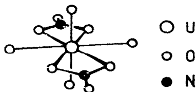
Fig. 21. View of the \text{UO}_2(\text{NO}_3)_2(\text{H}_2\text{O})_2 unit in the complex \text{UO}_2(18\text{-crown-6})(\text{NO}_3)_2 \cdot 2 \text{H}_2\text{O} .
